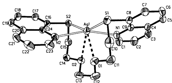
Fig. 3 Cationic structure of complex 2. Details as in Fig. 2.
