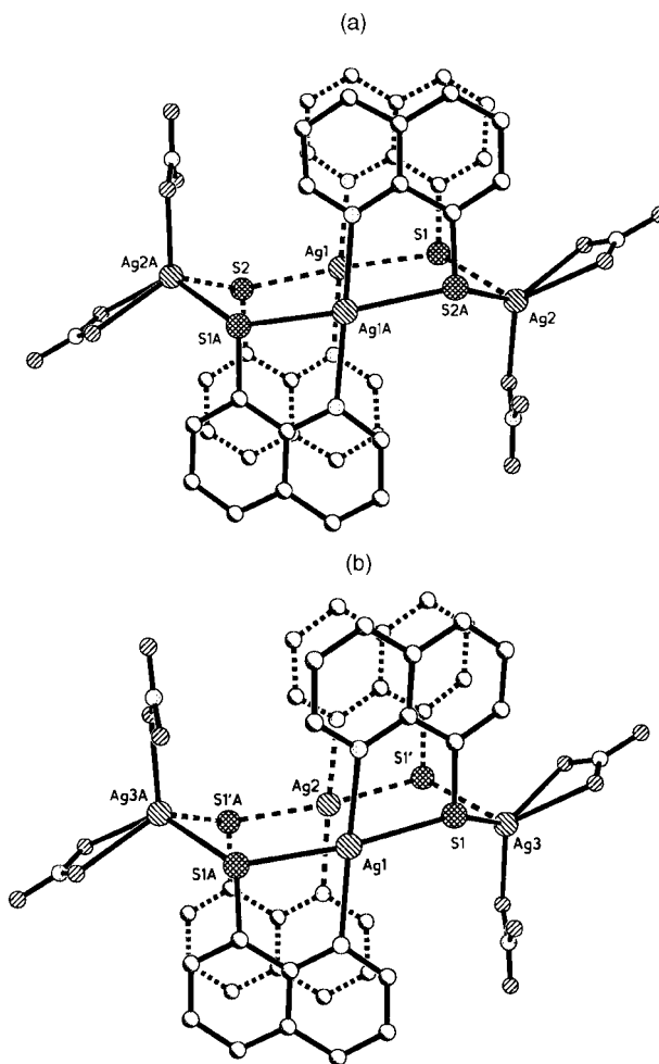
Fig. 7 Side view of the box-like [Ag 4 (ODSQ) 2 (NO 3 ) 4 ] 3 (a) and [Ag 4 (OESQ)(ODSQ)(NO 3 ) 4 ] 4 (b) showing the chair-like central ring Ag 4 S 4 . The polyethylene glycol backbones are omitted for clarity.
